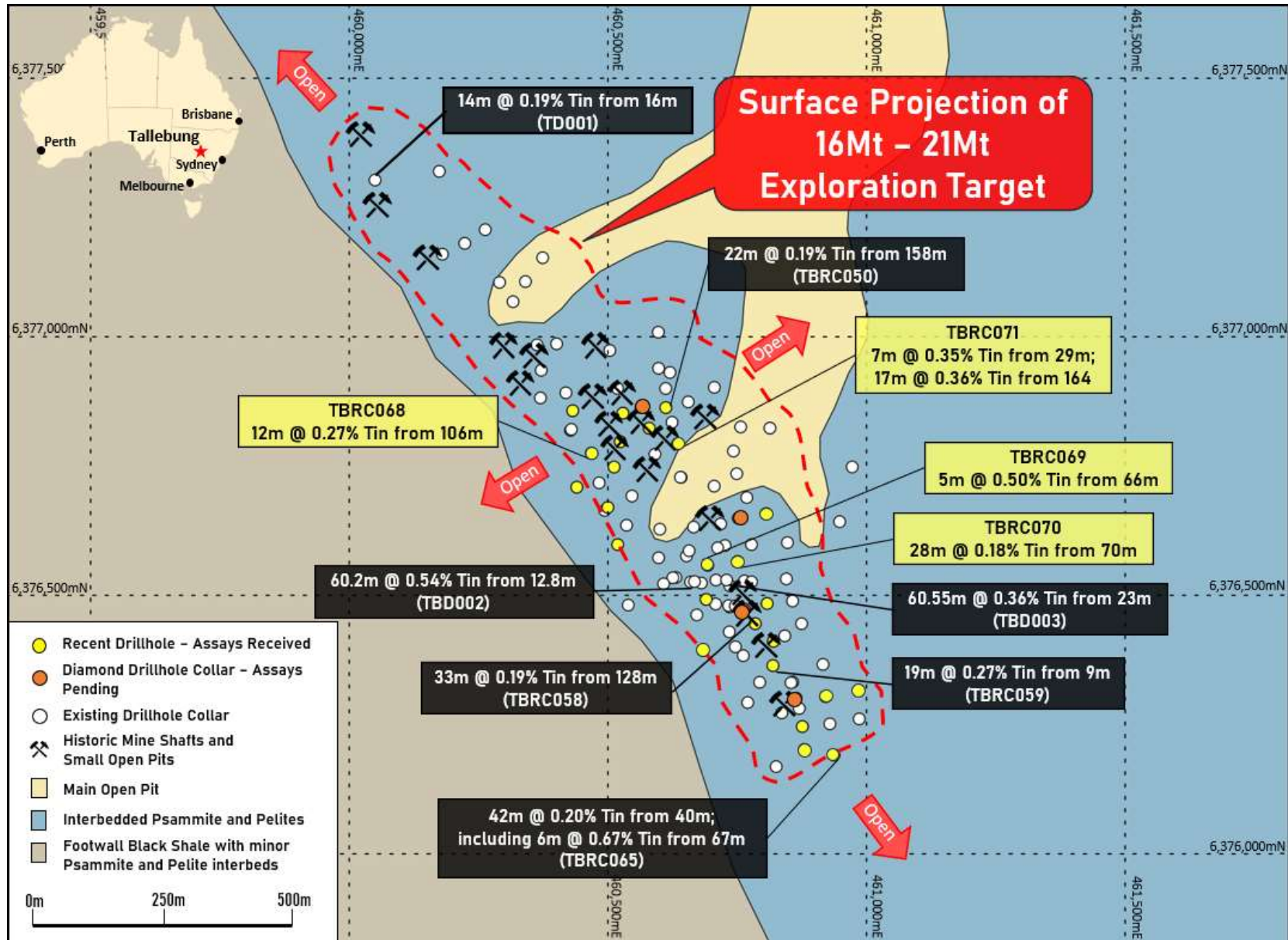
Figure 1: Tallebung Tin Project – Plan showing extent of the current Exploration Target along with locations of recently completed holes in the resource expansion and infill drilling program, overlaid on the geological map. New assays are in yellow.
